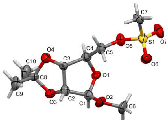
Figure 3. Molecular view and atom-labeling scheme for the X-ray structure of methyl 2,3-O-isopropylidene-5-O-mesyl- \beta -D-ribofuranoside. Displacement ellipsoids drawn at the 50% probability level.
