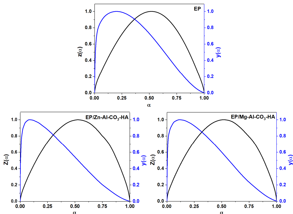
Figure A5. y(\alpha) and Z(\alpha) curves as a function of \alpha for prepared samples based on the Málék model.
