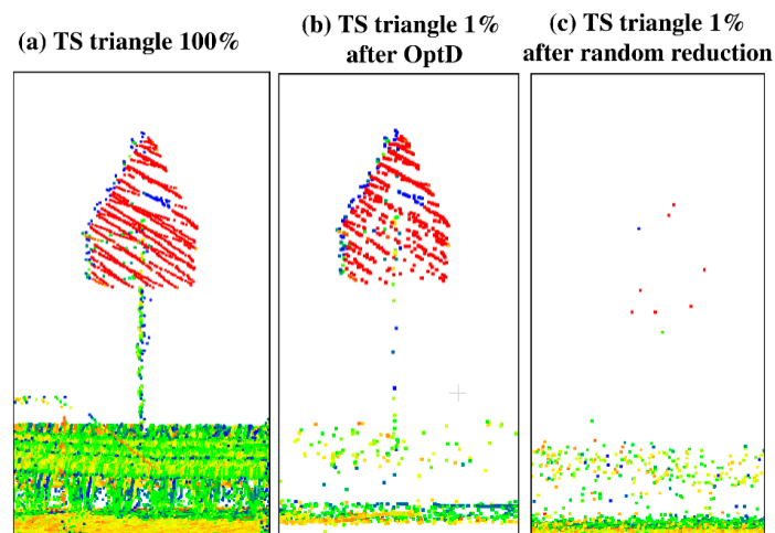
Figure 9. Data reduction effect on a triangular TS: (a) original, (b) triangular TS after OptD method, (c) triangular TS after random reduction.
