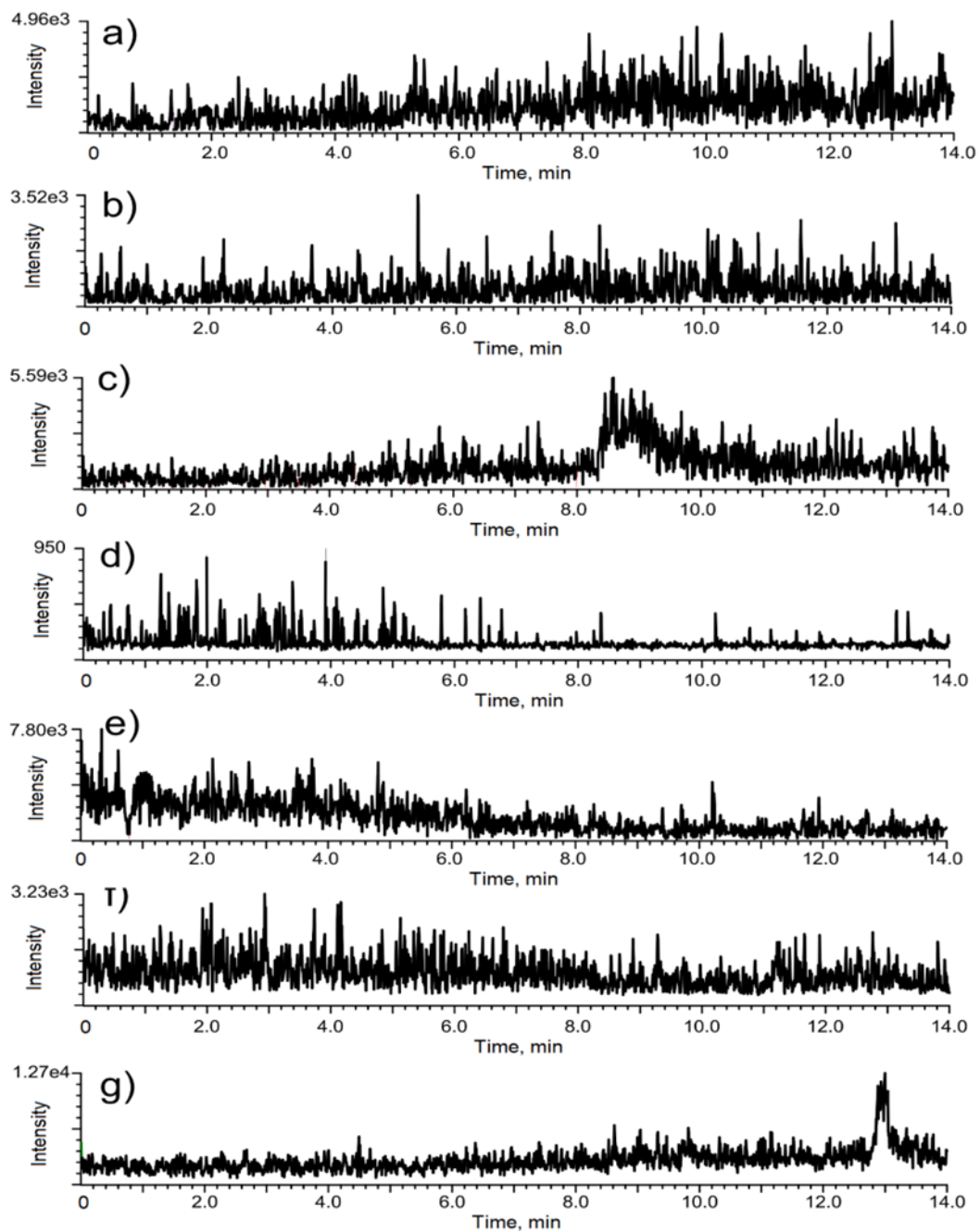
Figure 5. Chromatograms of a blank corresponding to the deep gas storage aquifer water sample (cf. Figure 4. measured for m/z (a) 135.9 → 93.0, (b) 193.0 → 149.0, (c) 120.9 → 77.0, (d) 144.0 → 99.1, (e) 207.0 → 163.1, (f) 135.0 → 91.0, (g) 221.1 → 177.1.
