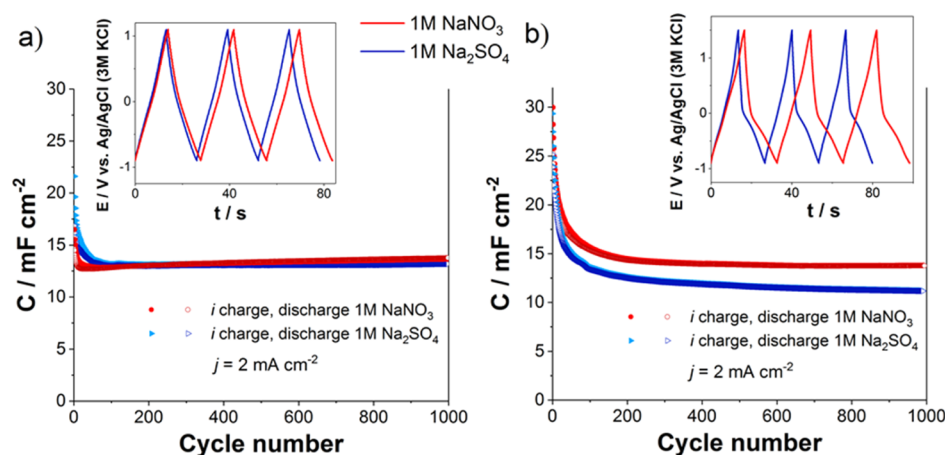
Figure 7. TiO 2 NT-BDD electrode capacitance as a function of cycle number in 1 M NaNO 3 and 1 M Na 2 SO 4 recorded in at various polarization ranges: (a) -0.9 to 1.1 V ( \Delta E = 2.0 V), (b) -0.9 to 1.5 V ( \Delta E = 2.4 V); current density: 2 mA cm -2 . Insets: the last cathodic and anodic branches (997–1000 cycle) of the chronopotentiometry curve.
