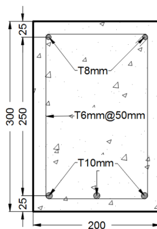
Fig.2: Beams details
