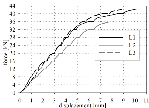
Fig. 4. Vertical force versus displacement up to rupture of lintels
