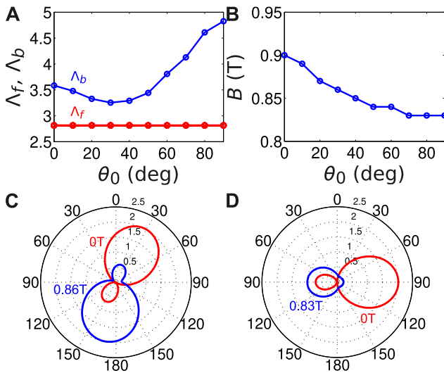
Figure 5: Study of the switching performance under oblique incidence of the impinging plane wave for R_1/R_2 = 0.9 , while R_2 = 10 \mu\text{m} and \lambda_b/R_2 = 8.04 . The external magnetic field is always z -directed.
