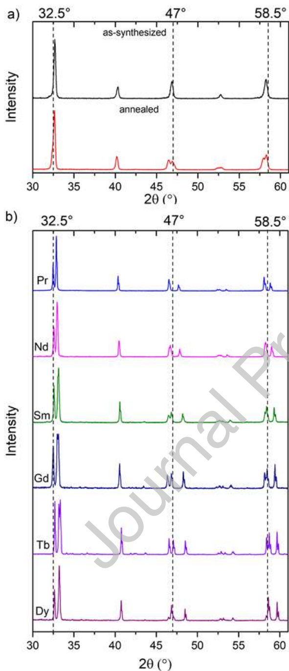
Figure 2. X-ray diffractograms of (a) pre- and post-annealed BaLaCo 2 O 6- \delta and (b) as-synthesised BaLnCo 2 O 6- \delta (Ln = Pr, Nd, Sm, Gd, Tb, Dy). The dotted lines are guides to the eye and mark the approximate positions of the
