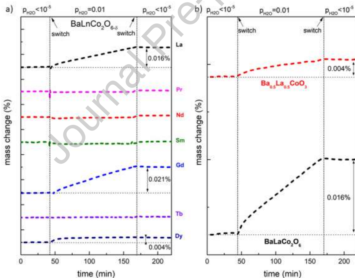
Figure 10. Water uptake in (a) BaLnCo_2O_{6-\delta} (Ln = La, Pr, Nd, Sm, Gd, Dy, Tb)
