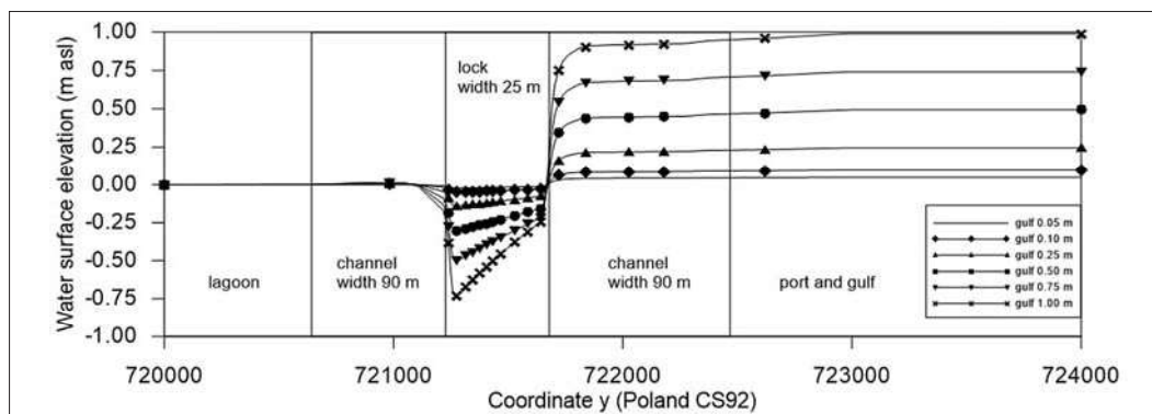
Fig. 6. Profiles of the water surface along the axis of the navigable channel (90 m wide) and lock (25 m wide) during the flow from the Gulf of Gdańsk to the Vistula Lagoon
