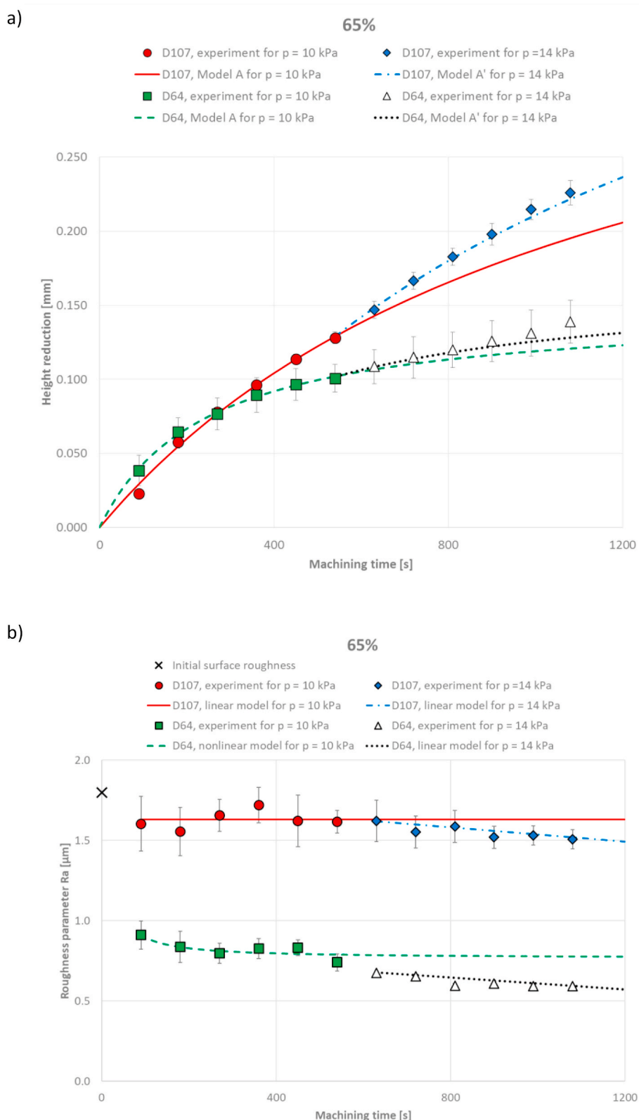
Fig. 3. Technological effects of lap-grinding of Al 2 O 3 ceramics using a diamond electroplated tool with the plating thickness corresponding to 65% of a nominal diamond crystal size: experimental and theoretical material removal (a) and surface roughness (b); see Table 1 for process parameters.
