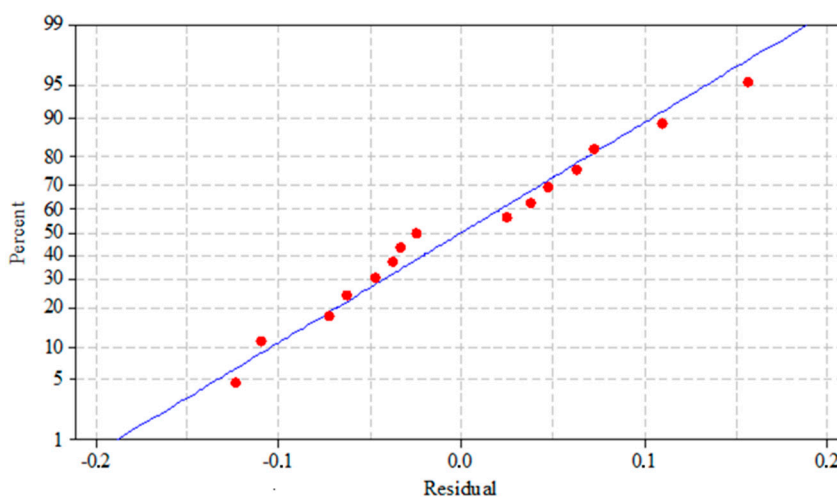
Figure 7. Normal probability plot of the residuals for surface roughness parameter of Ra.
