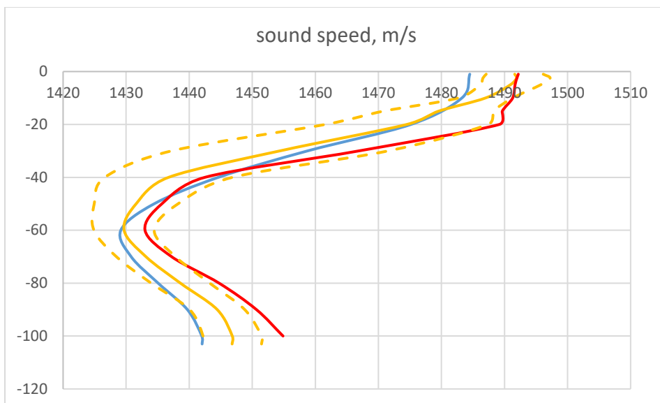
Fig. 11. Vertical temperature, salinity and speed of sound distributions in the Gdansk Deep region in August 2019 (red line) in comparison with the mean value (orange line) and confidence interval (dashed orange lines) determined for the period of 2010-2019 and the average for the period of 1960-2010 (blue line)
