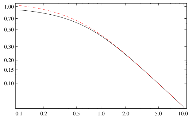
Figure 1. Log-log plots of \text{Exp}(-x) for \kappa_1 = 1, \kappa_2 = 0 (black), and \kappa_1 = \kappa_2 = 1 (red). The tails are identical.
