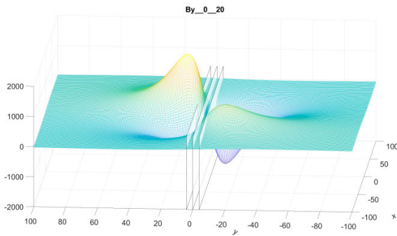
FIGURE 8. Field of B_y component expressed in nT, with cutting planes along P, K and S coordinates.
