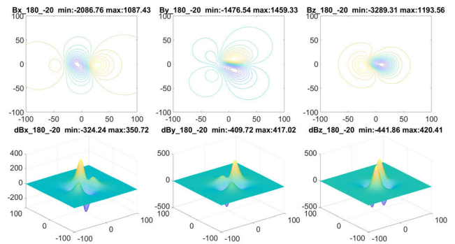
FIGURE 25. Ref-model differences on fields in nT: S1, direction 180.
