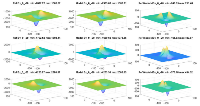
FIGURE 10. Ref-model differences on fields in nT: direction 0.
