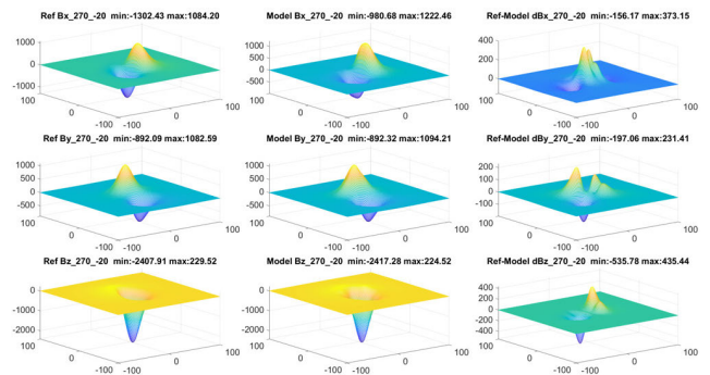
FIGURE 11. Ref-model differences on fields in nT: direction 270.
