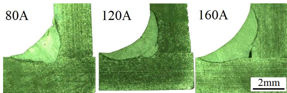
Fig. 6 Effect of welding current on the weld geometry – specimens from group E
