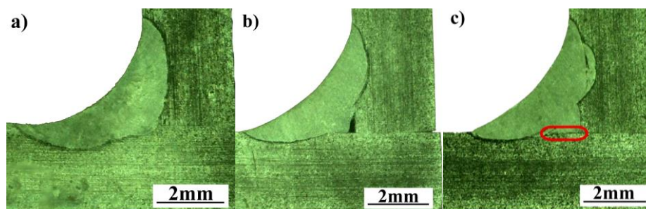
Fig. 7 Results of macroscopic tests; a) specimen D2, b) specimen E3, c) specimen G3, lack of fusion mark by red ellipse
