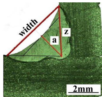
Fig. 5 The methodology of weld geometry measurements
