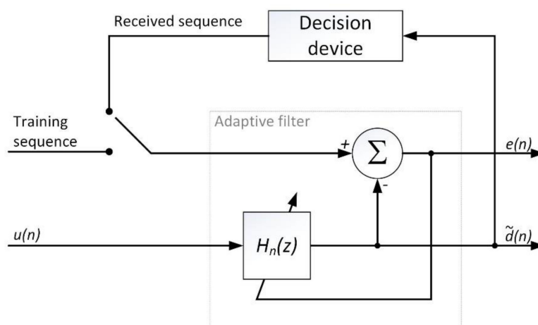
Figure 2. Adaptive channel correction system.
