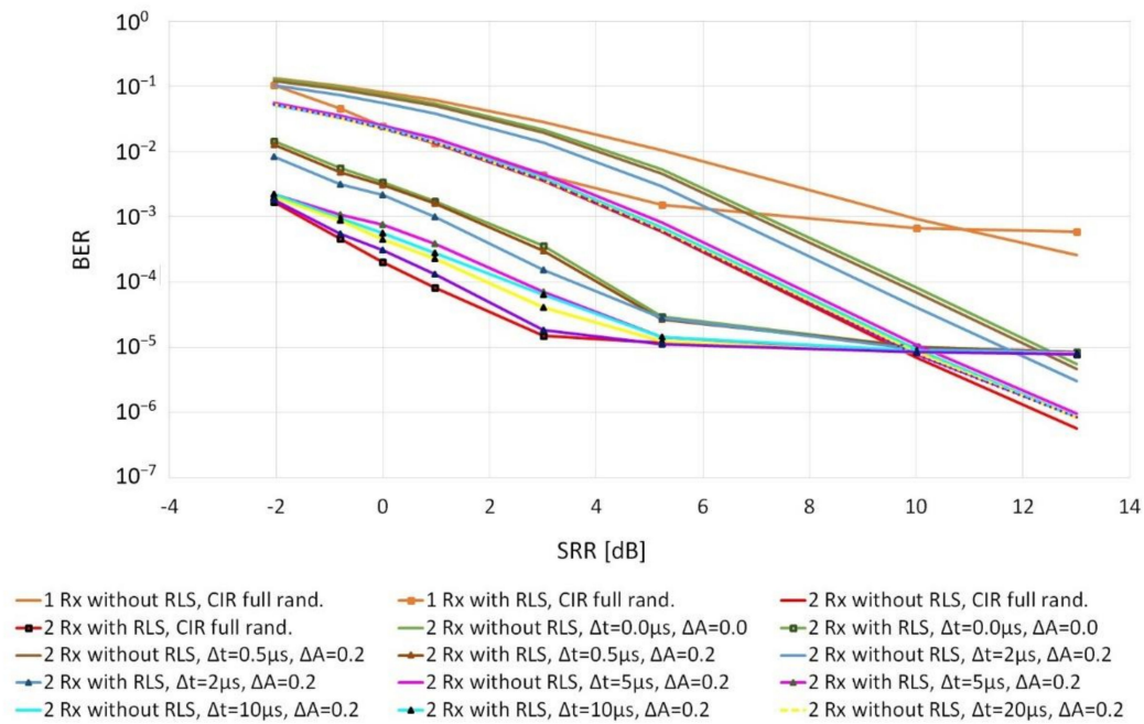
Figure 9. Impact of the differentiation of impulse responses on the quality of diversity combining when using two receivers for SNR = 10 dB and 4 replicas.
