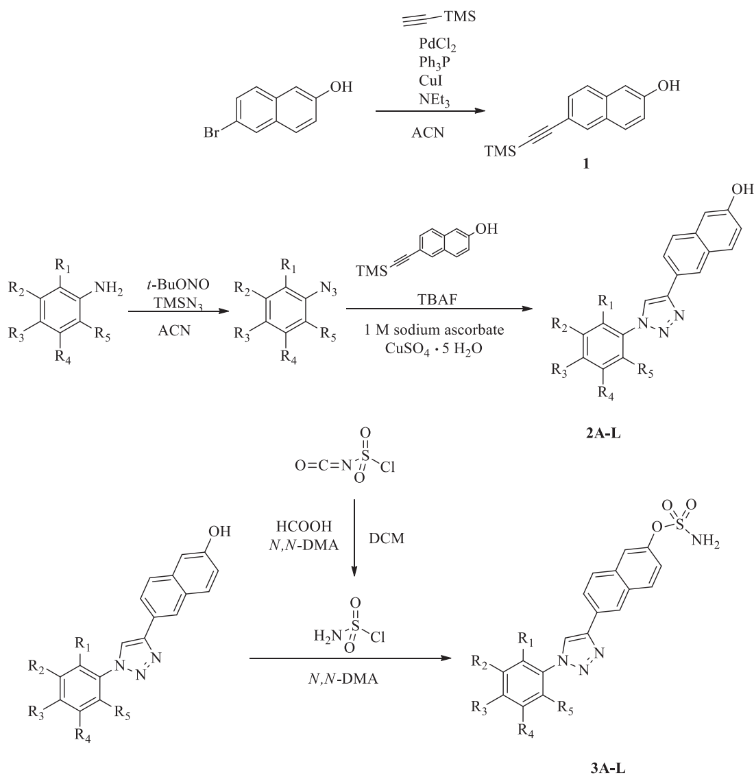
Scheme 1. Synthesis of 6-((trimethylsilyl)ethynyl)naphthalen-2-ol 1 and 6-(1-phenyl-1 H -1,2,3-triazol-4-yl)naphthalen-2-yl sulphamate derivatives ( R_1, R_2, R_3, R_4, R_5 = \text{H, F, Cl, or Br} ) 3A-L .
