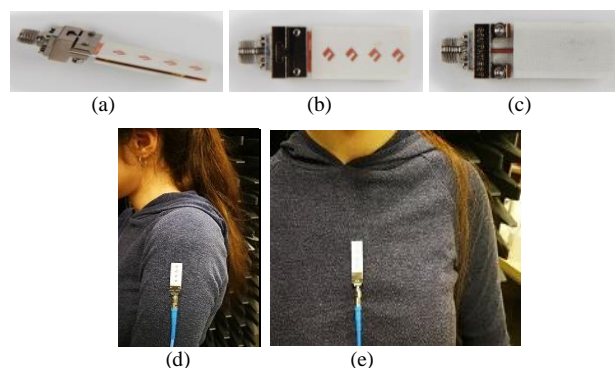
Fig. 3. Antenna prototype and characterization: (a) perspective view, (b) front view, (c) rear view, (d) antenna on-arm, (e) antenna on-chest.
