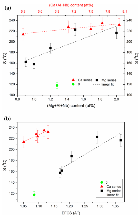
Figure 5 Comparison of glass stabilities S as a function of a (Mg + Nb + Al) for series Mg glasses or (Ca + Nb + Al) content for series Ca glasses and b ECFS for series xMg and xCa glasses. Dashed lines show trends of thermal properties and are given as guide for the eyes only.
