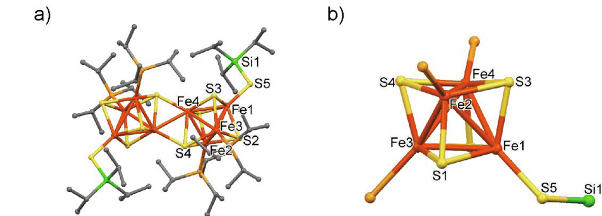
Fig. 24. Molecular structures of the supramolecular iron(II) silanthiolates (Part I); H atoms are omitted: a) [(i\text{Pr}_3\text{P})_4\text{Fe}_8\text{S}_8(\text{SSiPh}_3)_2] [139]; b) [(i\text{Pr}_3\text{P})_3\text{Fe}_4\text{S}_4(\text{SSi}i\text{Pr}_3)] – isopropyl substituents at P and \text{Si}i\text{Pr}_3 groups are omitted for clarity [140].
