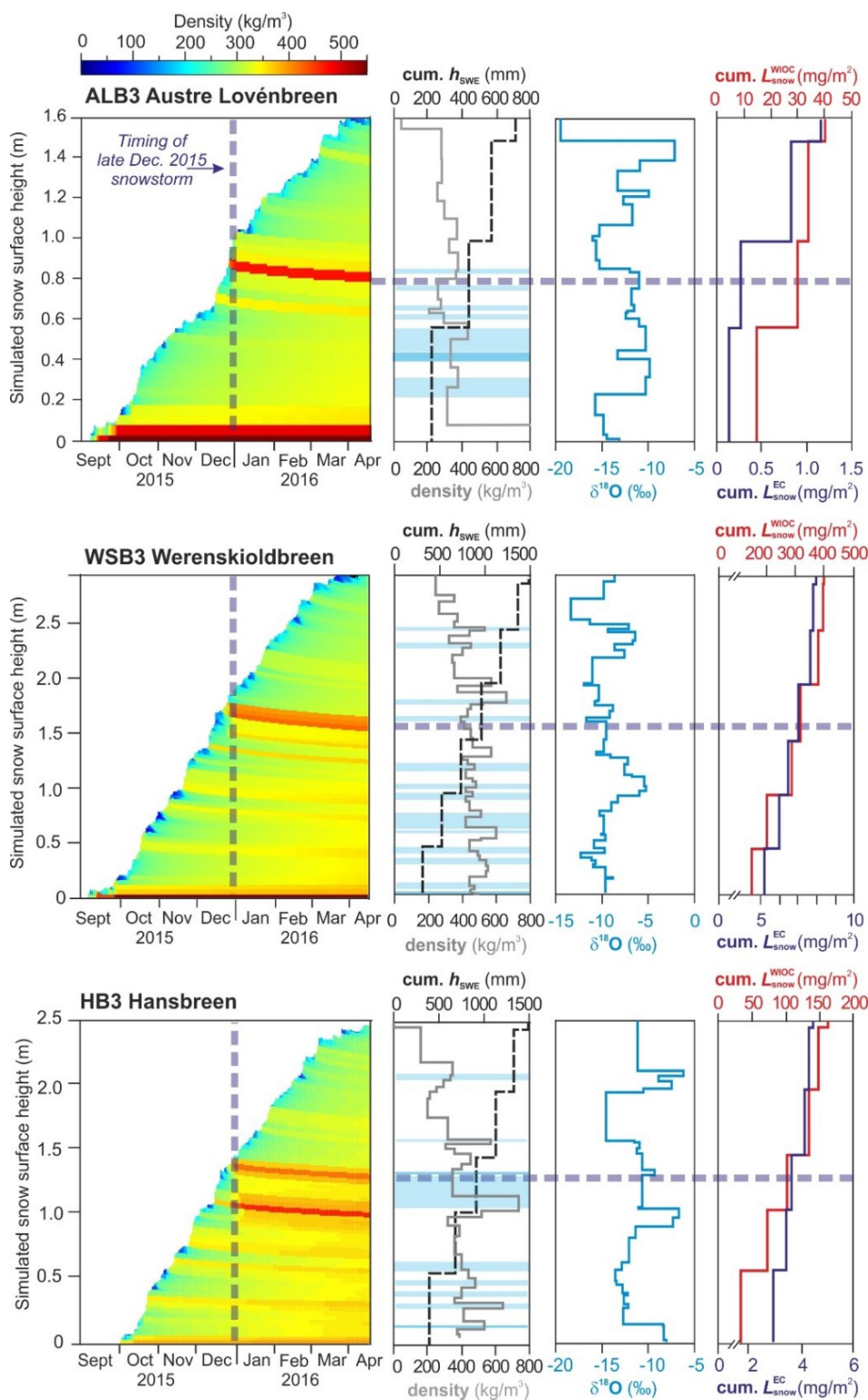
Figure 8. Simulated evolution of the snowpack from September 2015 to April 2016 at three glacier sites on Spitsbergen, compared with measured profiles of density, cumulative h_{SWE} , \delta^{18}O , as well as cumulative L_{snow}^{EC} and L_{snow}^{WIOC} in the snowpack. The h_{SWE} over the EC and WIOC sampling intervals was computed using the discrete snow layer density data. Where density measurements were missing, values from comparable layers in other snowpits were used. Snow layers with C_{snow}^{EC} < 1 \text{ ng g}^{-1} were assigned a value of 0.5 \text{ ng g}^{-1} for L_{snow}^{EC} calculations. Icy snow and discrete ice layers are shown as pale and darker blue lines, respectively.
