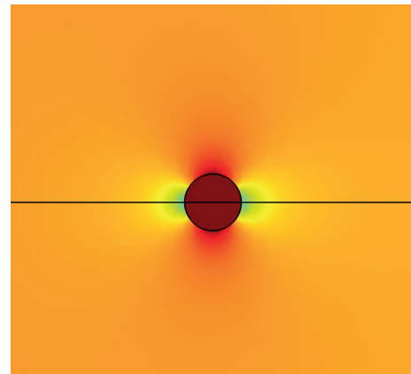
Fig. 14. Electric field distribution of the 50 μm gas-filled spherical void inside the 3 mm spherical protrusion located at the conductor screen
