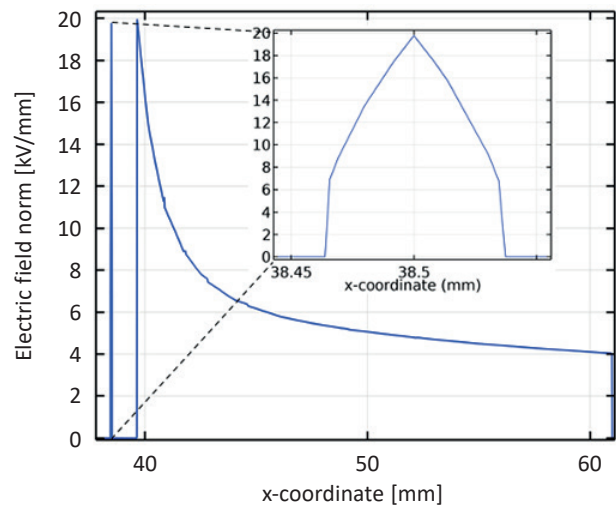
Fig. 15. Electric field plot of the 50 μm gas-filled spherical void inside the 3 mm spherical protrusion located at the conductor screen
