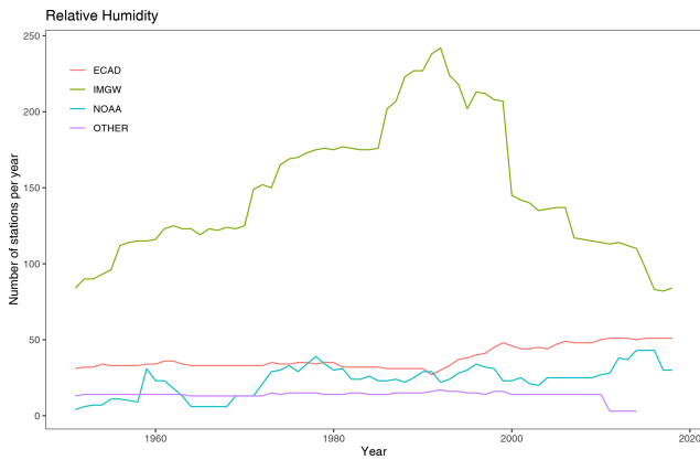
Figure 4. Number of meteorological stations for relative humidity observations per year from 1951 to 2019.
