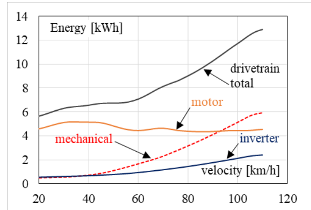
Fig. 7. Relation between drivetrain energy losses and cruising velocity (running in cruising mode)
