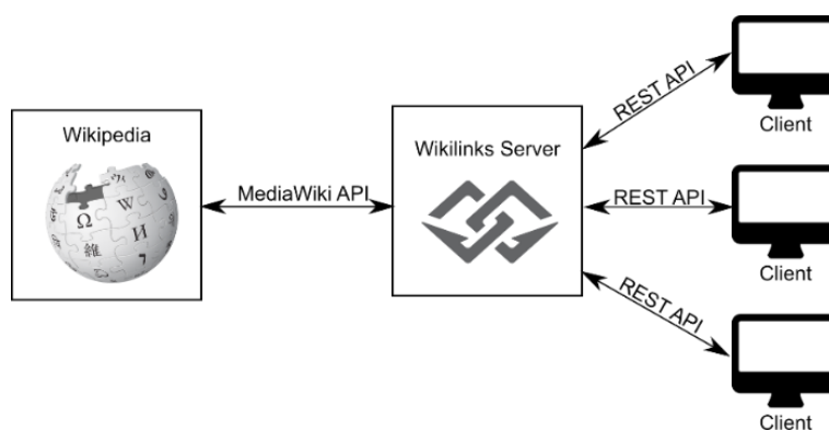
Figure 1: The architecture of WikiLinks
