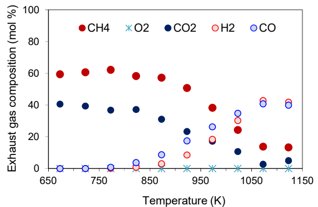
Fig. 4 Biogas reforming on Rh/Cu-CeCa sample: (a) CH 4 and CO 2 conversion; (b) exhaust gas composition as a function of reaction temperature. W/F = 13 g at h/mol.
