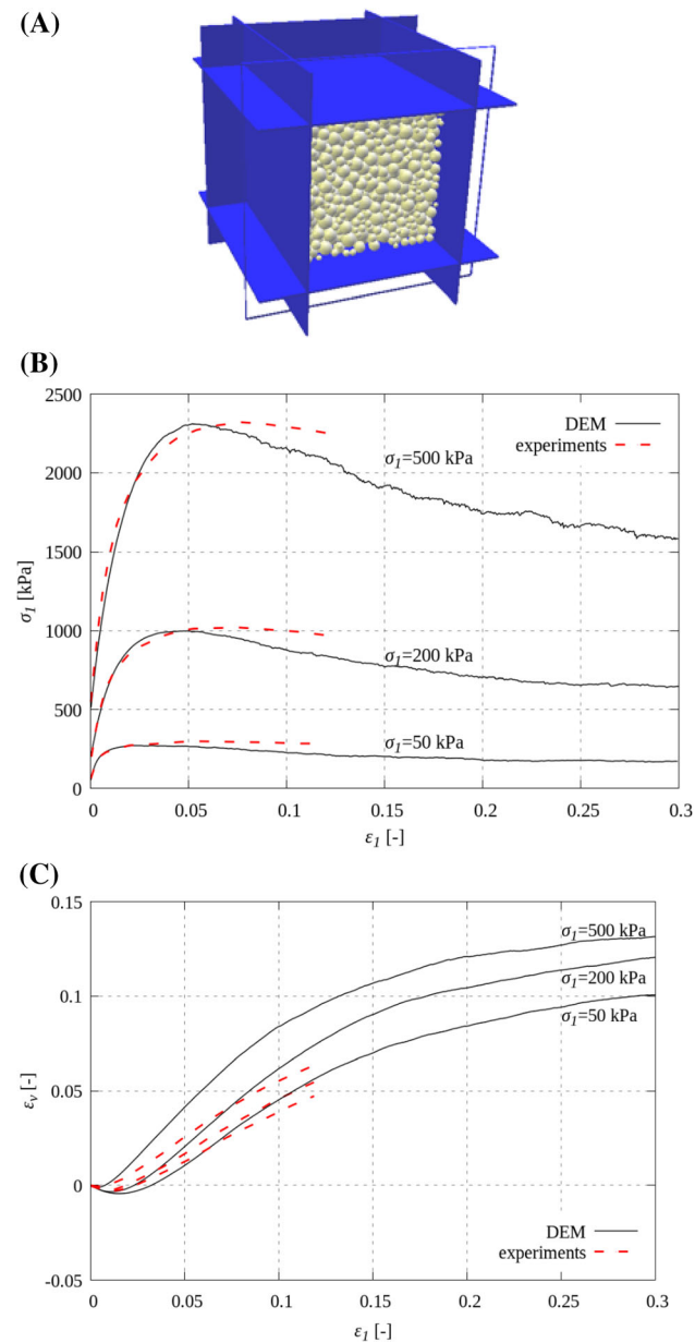
Fig. 3 Triaxial compression test on initially very dense sand (initial void ratio e_o = 0.53 ) using clumps: a DEM model set-up and b calculated vertical normal stress \sigma_v and c calculated volumetric strain \epsilon_v versus vertical normal strain \epsilon_1 from DEM compared to laboratory experiments [26] for different initial lateral pressure: \sigma_c = 50 kPa, \sigma_c = 200 kPa and \sigma_c = 500 kPa
