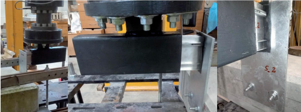
Fig. 3. View on laboratory test stand
