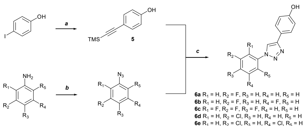
Scheme 1. Synthesis of 4-(1-phenyl-1H-1,2,3-triazol-4-yl)phenol derivatives 6a–e : (a) ethynyltrimethylsilane, PdCl 2 , Ph 3 P, CuI, NEt 3 , ACN; (b) t -BuONO, TMSN 3 , ACN; (c) TBAF, sodium ascorbate, CuSO 4 ·5H 2 O.
