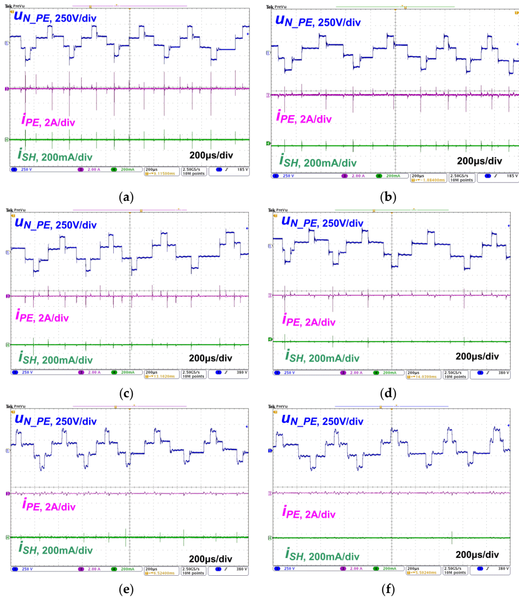
Figure 28. Experimental waveforms of CM voltage u_{N\_PE} , leakage current i_{PE} and shaft-grounding brush current i_{SH} measured in a configuration with a 1 m cable for: (a) inverter; (b) motor choke; (c) du/dt choke; (d) sine-wave filter; (e) CM choke; (f) CM choke with sine-wave filter.
