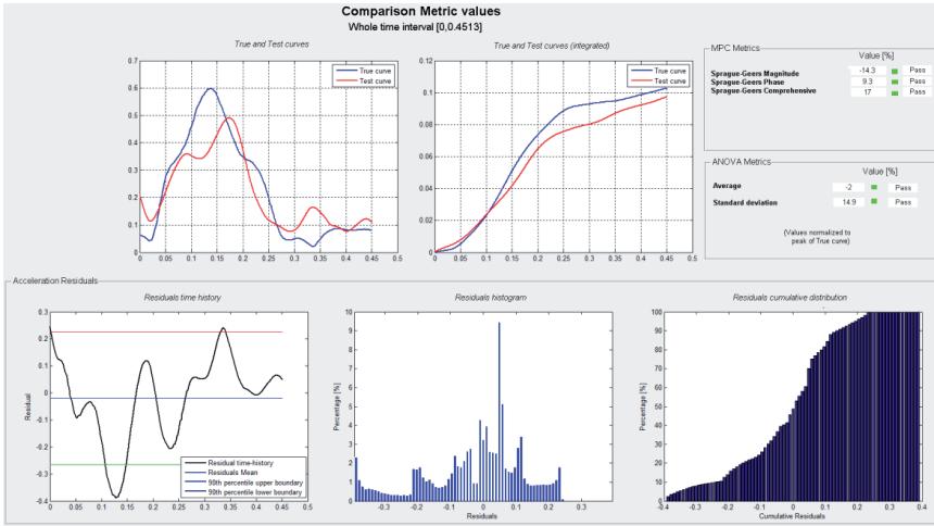
Fig. 6. Comparison of ASI curves using RSVVP code: blue — full-scale crash test; red — simulation
