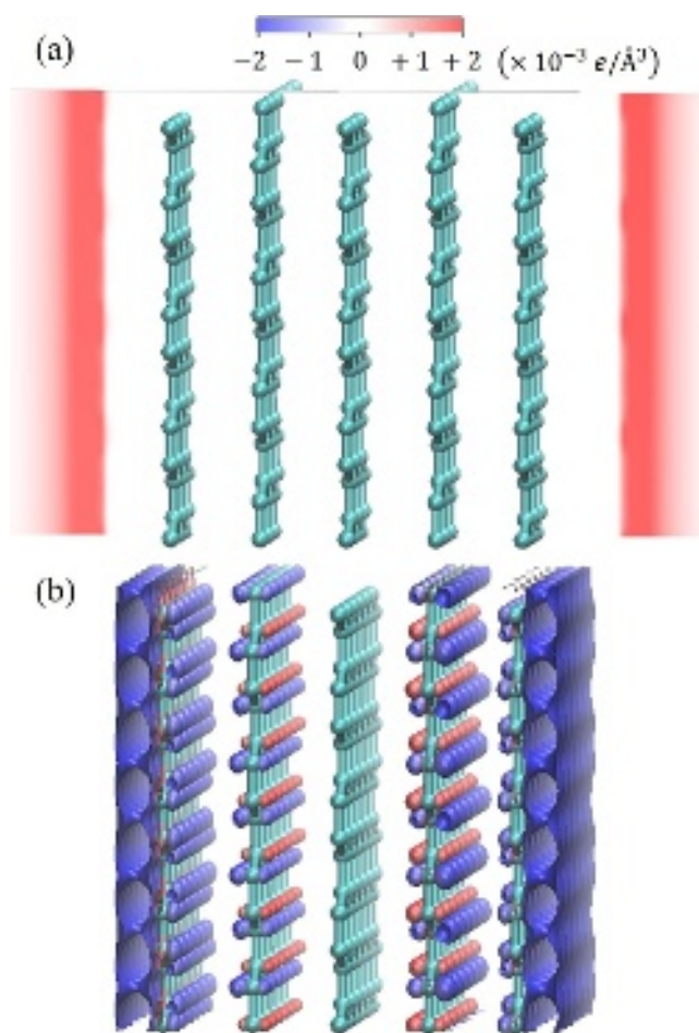
Figure 10: Difference in charge densities of a system at U = 1.0 \text{ V} (with respect to \text{Li}^+/\text{Li} ) from a system at U = 0.0 \text{ V} (with respect to \text{Li}^+/\text{Li} ). (a) Electrolyte density \rho_d in a plane bisecting the 5-layer graphene sheet orthogonally, (b) Electronic density isosurfaces at \rho_e(\mathbf{r}) = \pm 2.0 \times 10^{-3} e/\text{\AA}^3 .
