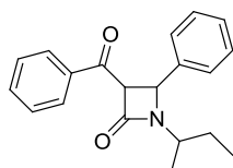
3-Benzoilo-1-(sec-butylo)-4-feniloazetydino-2-on, (104aaa), (104'aaa)
