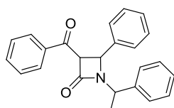
3-Benzoilo-4-fenilo-1-(1-feniloetylo)azetydino-2-on, (104aaa), (104'aaa)
