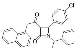
4-(4-chlorofenylo)-3-((naftalen-1-ylo)acetylo)-1-(1-fenyloetylo)azetyldyno-2-on, (104bba), (104'bba)
