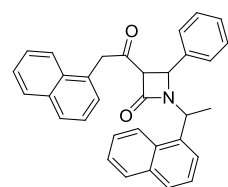
3-((Naftalen-1-ylo)acetylo)-1-(1-(naftalen-1-ylo)etylo)-4-fenyloazetyldyno-2-on, (104bab), (104'bab)
