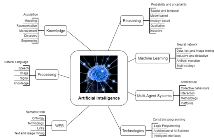
Fig. 1. Artificial Intelligence 3.0 [55].
