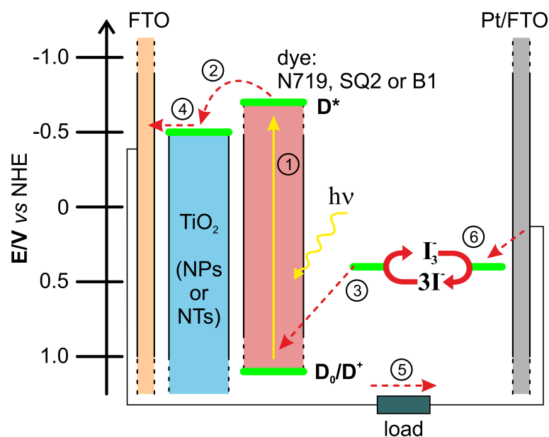
Figure 3.2. Energy level diagram and principles of operation of a DSSC
