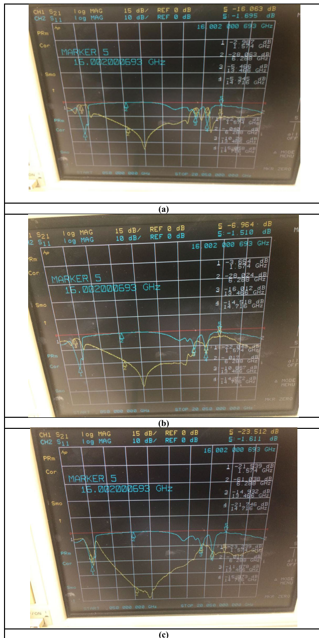
FIGURE 17. The photos of the utilized network analyzer screen during the measurement process of (a) S_{11} and S_{12} , (b) S_{11} and S_{13} , and (c) S_{11} , and S_{14} parameters.
