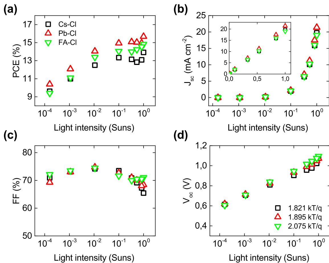
Figure 7: Four photovoltaic parameters versus light intensity drawn for representative solar cell devices obtained with different sources of chlorine atoms, (a) PCE, (b) J_{sc} , (c) FF, (d) V_{oc} . The ideality factors for all samples are written in part (d).
