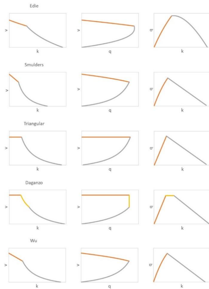
Figure 2. Relationships v(k) , v(q) , and q(k) in selected multi-regime models (assuming model continuity).
