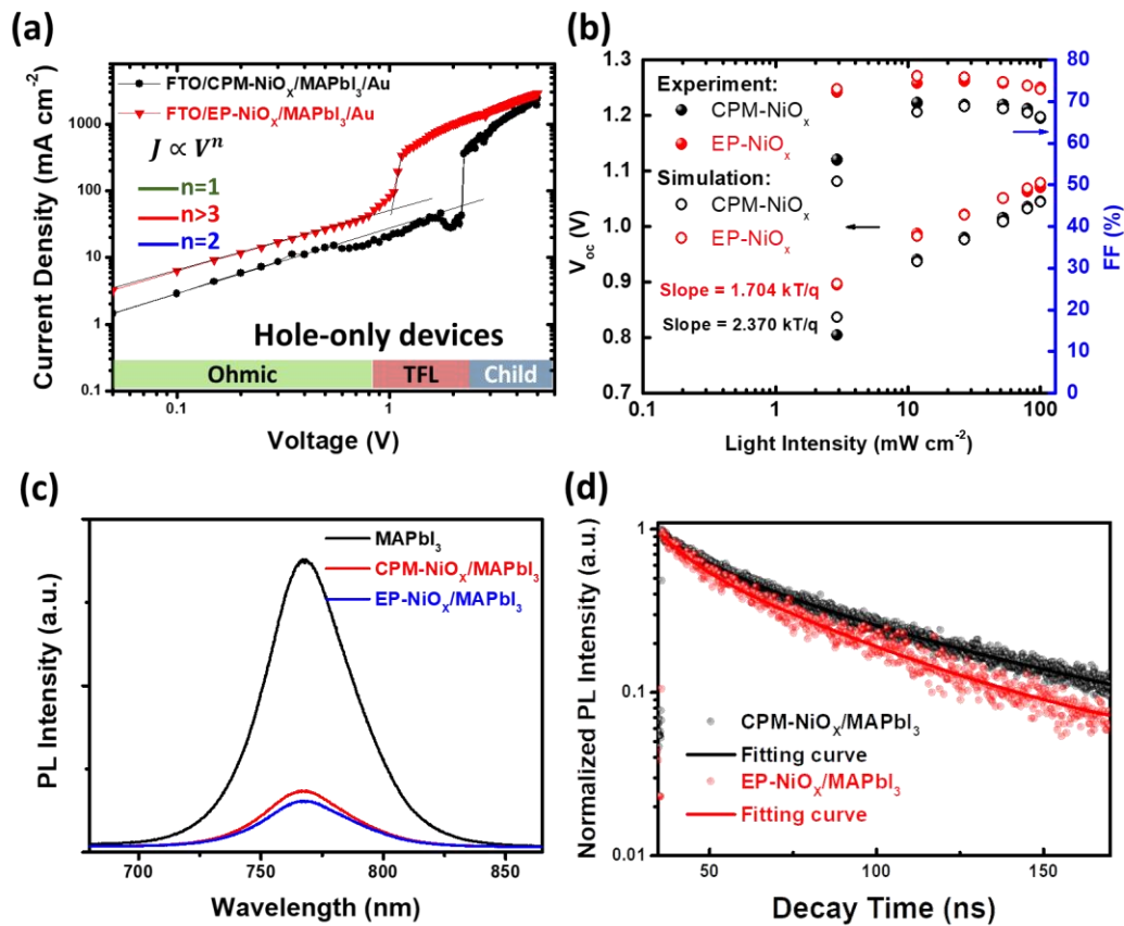
Figure 6. (a) SCLC measurement of hole-only device and (b) photovoltaic parameters of V_{oc} , and FF measured under different light intensities for PVSCs fabricated from CPM- NiO_x and EP- NiO_x films. (c) Steady-state PL and (d) TRPL spectrum of perovskite films deposited on CPM- NiO_x and EP- NiO_x film.
