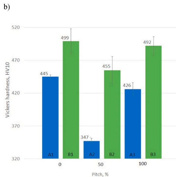
Fig. 8. Comparison of average values of hardness with different values of the pitch and standard deviation bars: a) in weld metal, b) in HAZ.
