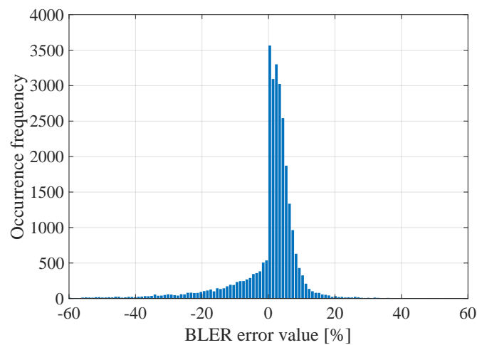
Figure 23. The BLER error histogram of the proposed DL model.
