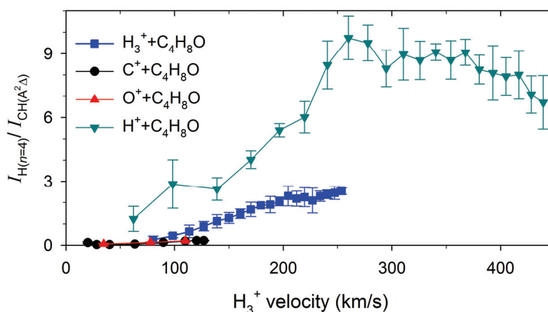
Fig. 4 – (Color online). The ratio of intensities of the \text{H}(n=4) and \text{CH}(A^2\Delta) fragments in the collisions of \text{H}_3^+ with tetrahydrofuran. The ratios obtained from the THF fragmentation induced by proton [20] and the \text{O}^+ and \text{C}^+ [19] impact are shown for comparison.
