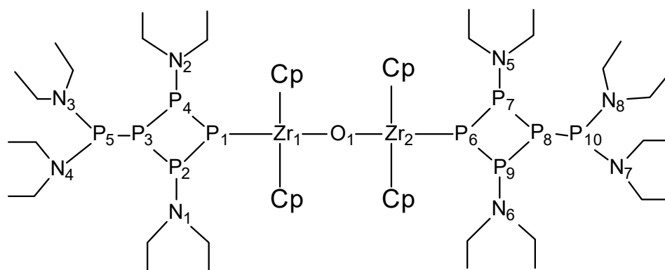
Figure 1. Structure of [[(\eta^5\text{-C}_5\text{H}_5)_2\text{Zr}[\mu\text{-P}(\text{NEt}_2)_2\text{P}(\text{NEt}_2)_2\text{P}]]_2\text{O} (1).
