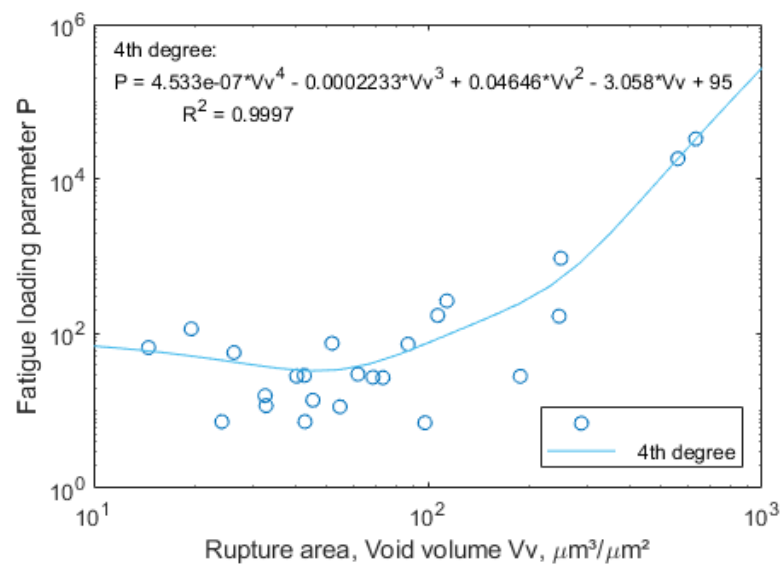
Figure 14. Fatigue loading parameter P vs. void volume Vv in the rupture area and their 4th degree fit.
