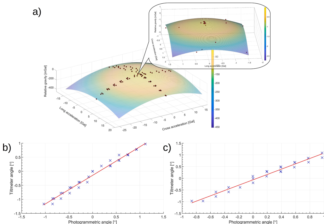
Fig. 3. The results of tiltmeters calibration: a) The parabolic surface fitted to the data in order to find where its maximum is located, the 2 Gal zone around maximum is magnified b) the calibration of the scale factor of long tiltmeter c) the calibration of the scale factor of cross tiltmeter.
