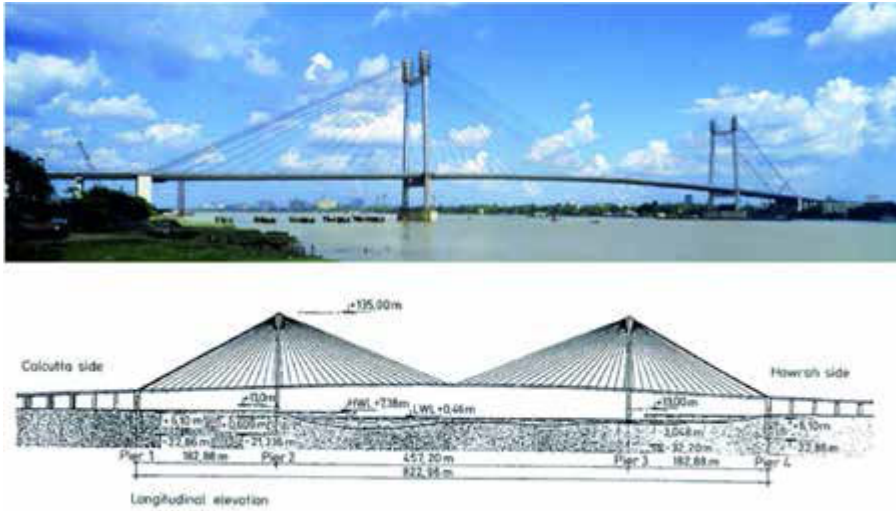
Fig. 14. Hooghly River Bridge, Kolkata, India, 1994 [5], (photo: wikipedia.com)
