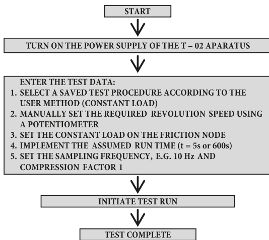
Fig. 7. Algorithm of tests on the measuring stand
