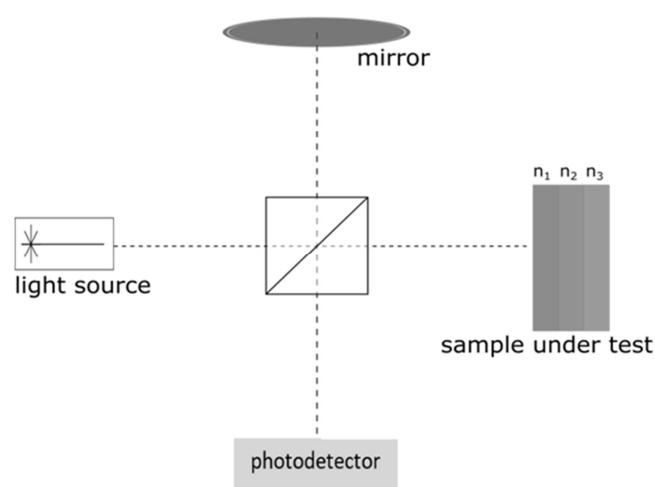
Fig. 1. OCT system diagram
