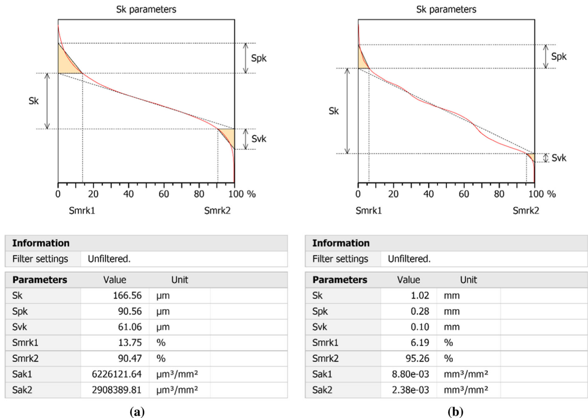
Fig. 14 Representation of functional (stratified) parameters in Abbott-Firestone curve for the specimen: a C6a; and b B3b
